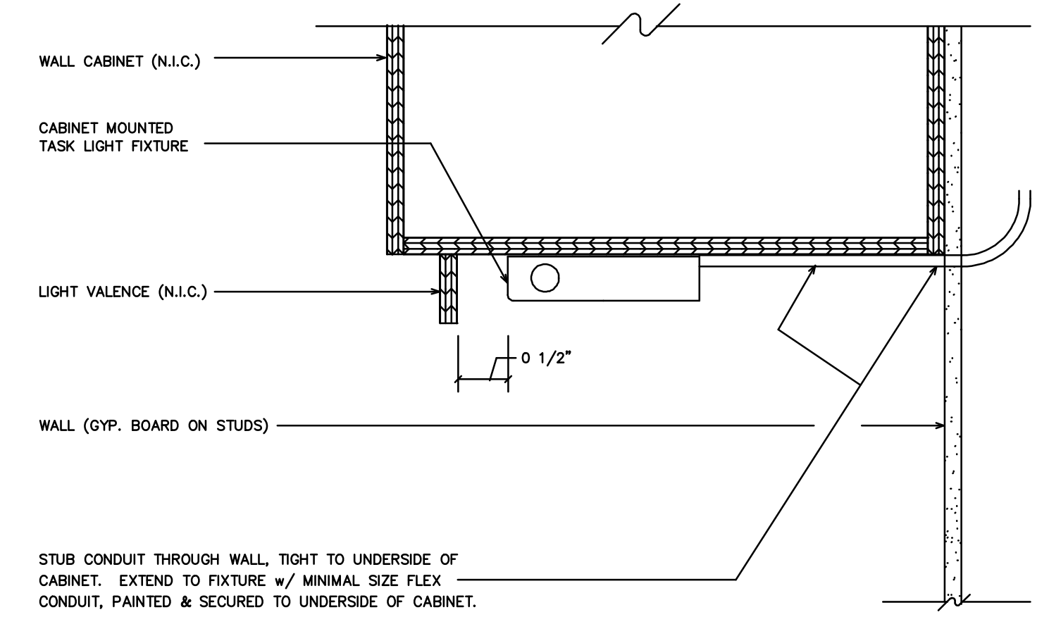
TASK LIGHT INSTALLATION DETAIL
